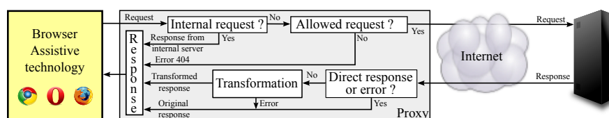
Fig. 1. Request processing by the proxy.
