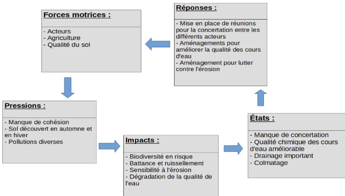
Figure 43: Diagramme DPSIR
