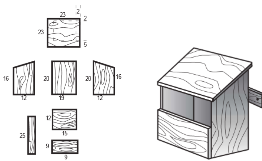
Figure 29-Nichoir semi-ouvert
