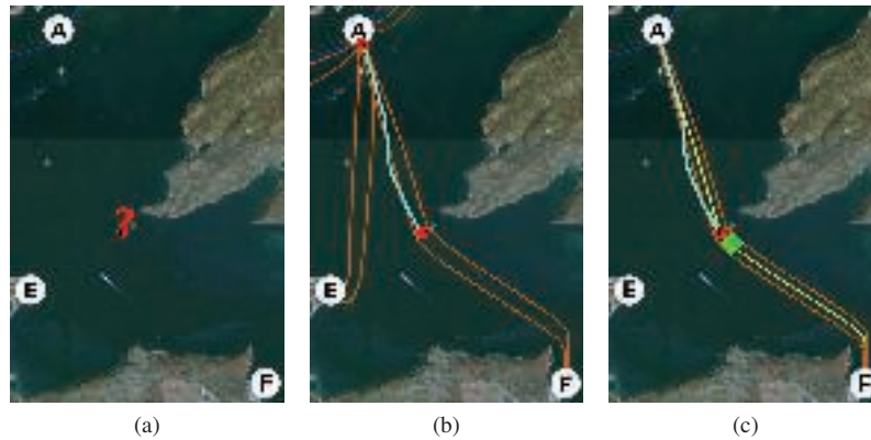
Figure 11.6 Outlier detection.
