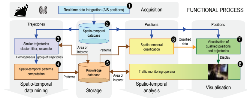
Figure 11.2 Data mining and trajectories' qualification process.
