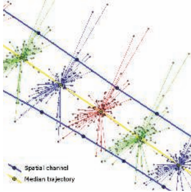
Figure 11.4 Clusters of positions and spatial pattern.
